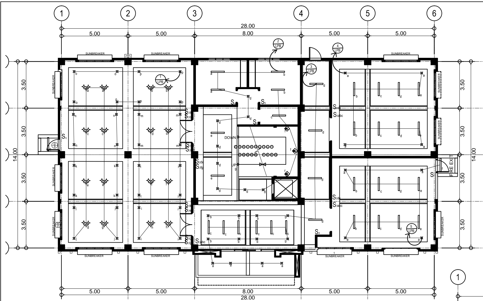
SECOND FLOOR LIGHTING LAY-OUT SCALE 1:100MTS
