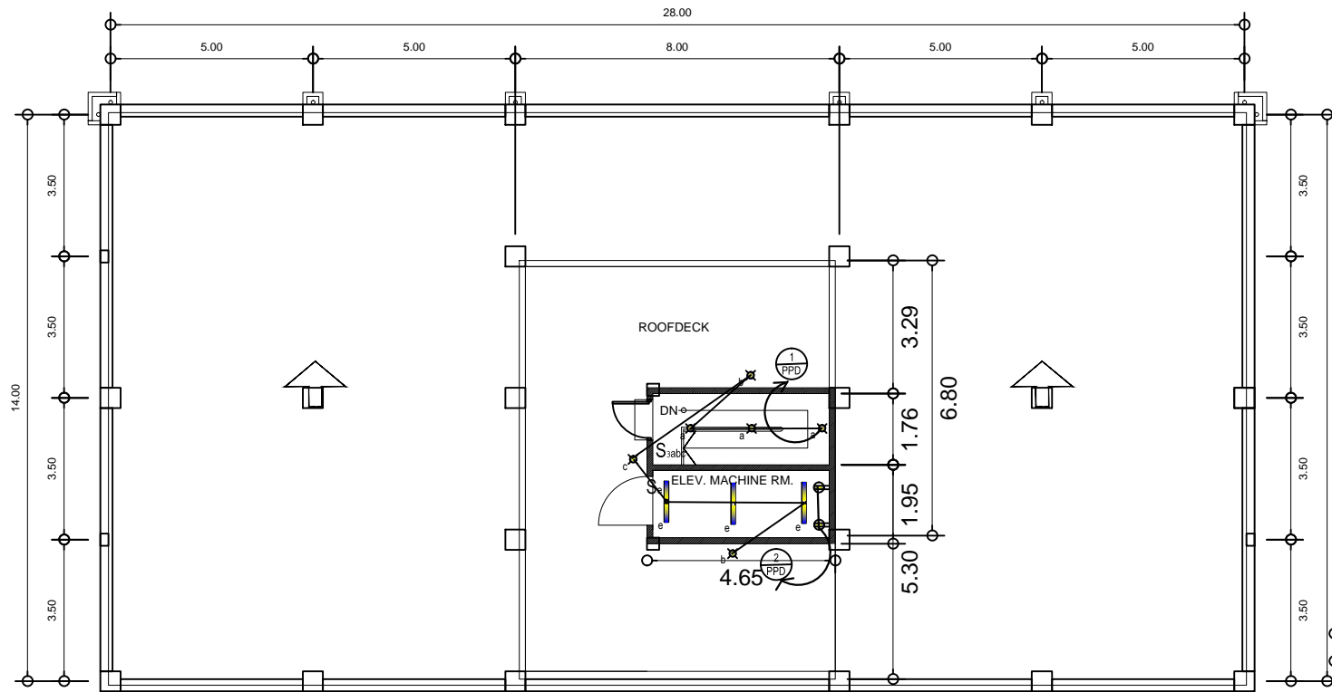
ROOF DECK LIGHTING LAYOUT SCALE 1:100MTS
