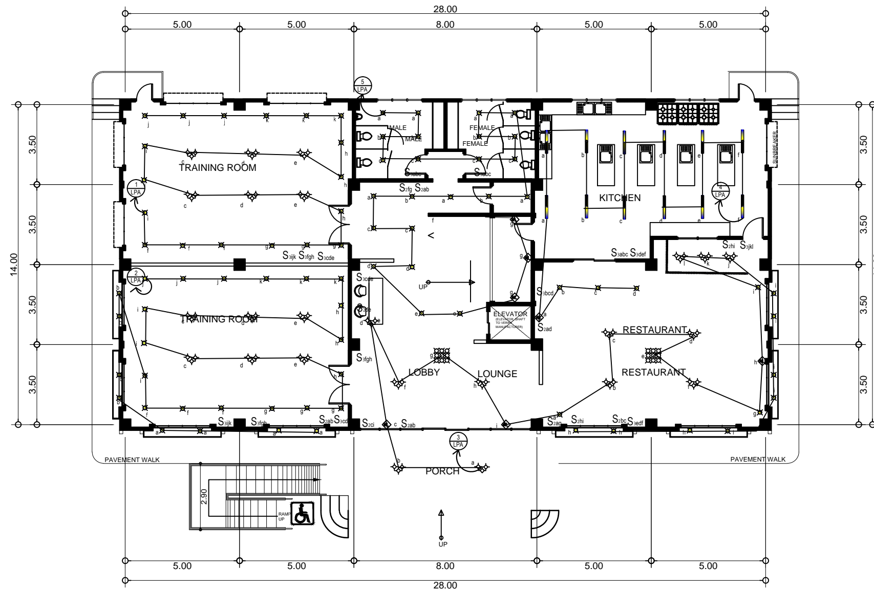
GROUND FLOOR LIGHTING LAY-OUT SCALE 1:100MTS
