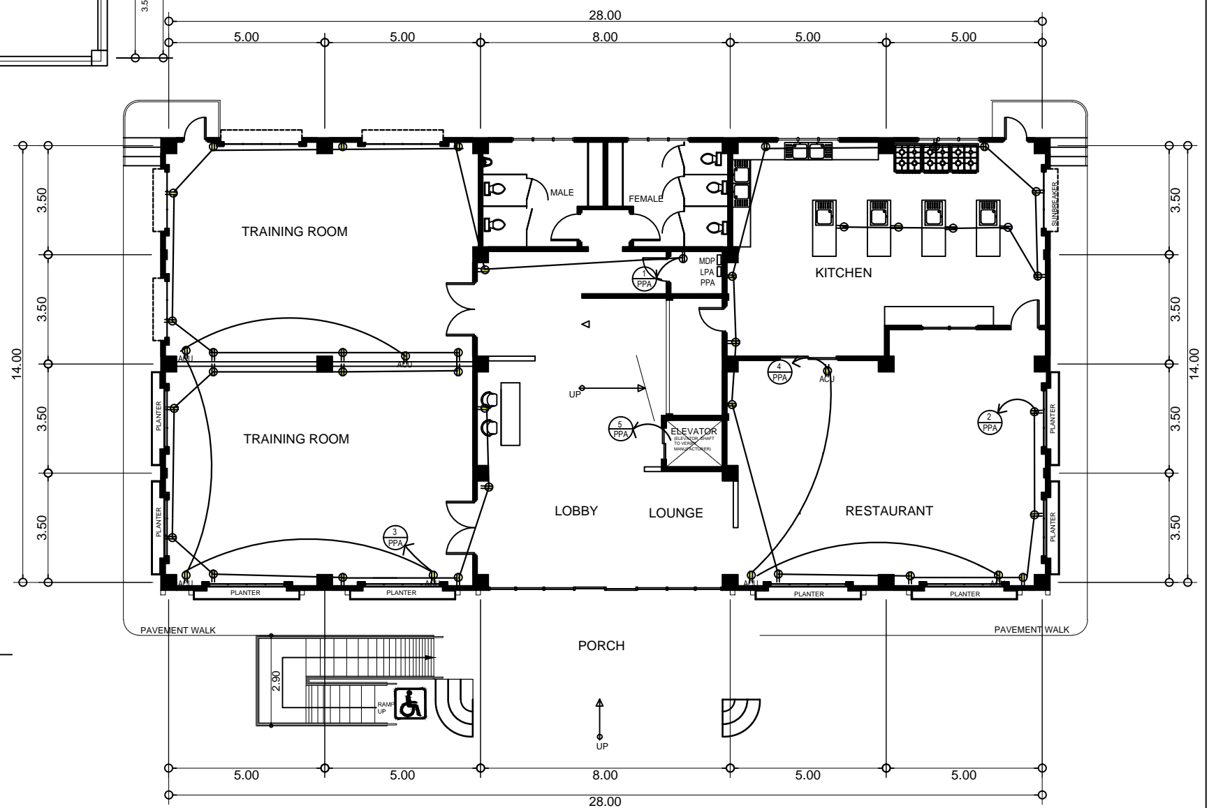
GROUND FLOOR POWER LAY-OUT SCALE 1:100MTS
