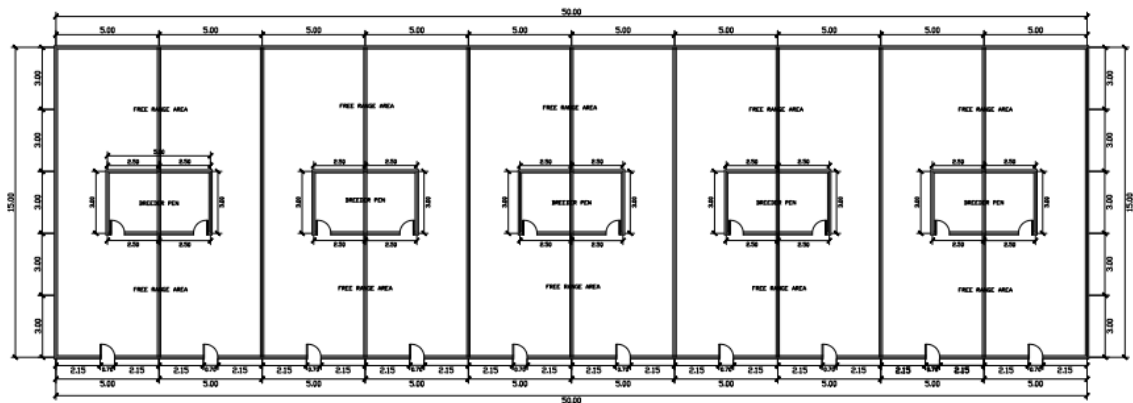
RANGE FLOOR PLAN SCALE: 1:150MTRS
